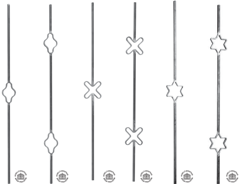
Art. 1324/1 \varnothing 12 x 12 mm H 1000 mm L 80 mm
