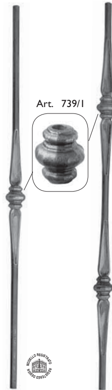
Art. 1177/1 Art. 1177/2 Ø 12 mm Ø 12 mm H 1000 mm H 1000 mm
