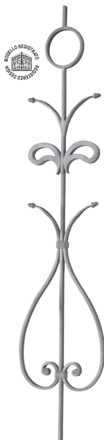
Art. GD192/1 □ 14 x 8 mm H 1000 mm L 225 mm
