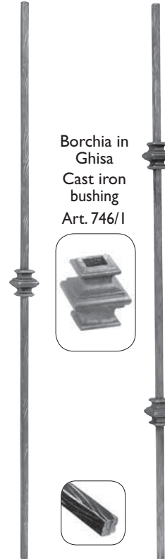
Art. 1175/3 Art. 1175/4 Ø 12 x 12 mm Ø 12 x 12 mm H 1000 mm H 1000 mm
