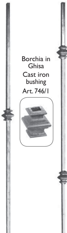
Art. 755/5 Art. 755/6 Ø 12 x 12 mm Ø 12 x 12 mm H 900 mm H 900 mm
